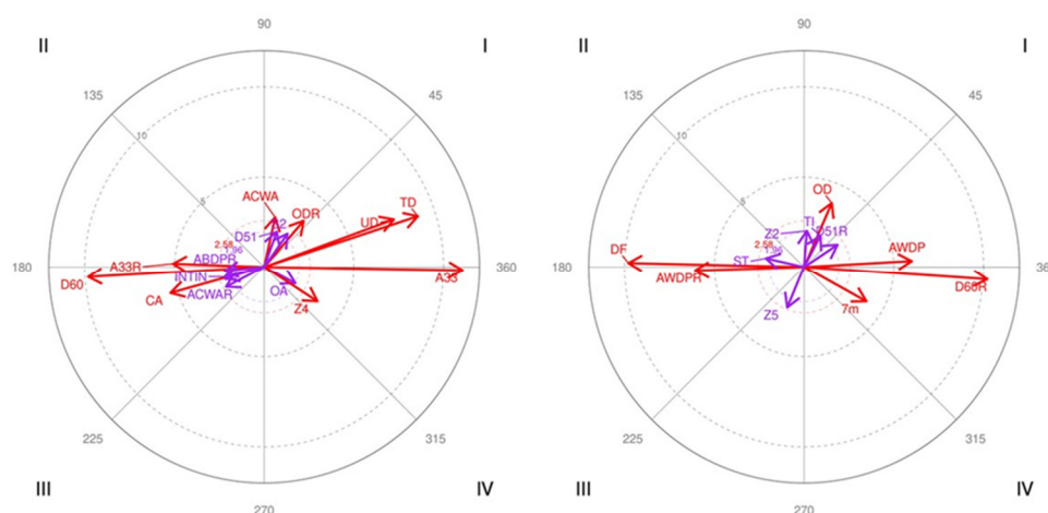
Figure 3. Vector maps for local behaviour FAILURE. I: Quadrant I; II: Quadrant II, III: Quadrant III; IV: Quadrant IV
