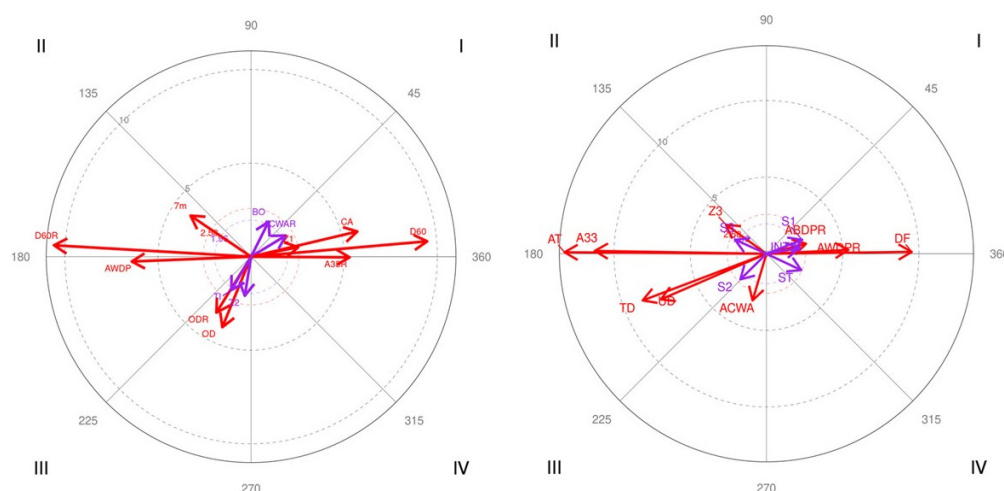
Figure 2. Vector maps for local behaviour SUCCESS. I: Quadrant I; II: Quadrant II, III: Quadrant III; IV: Quadrant IV
